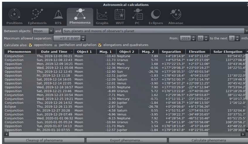
Figure 4.32: Astronomical Calculations (AstroCalc): Phenomena
