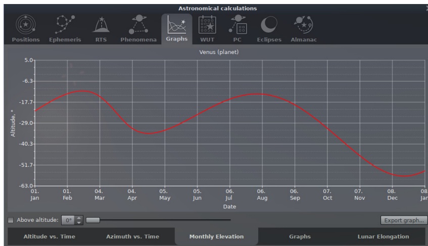
Figure 4.35: Astronomical Calculations (AstroCalc): Graphs / Monthly Elevation
