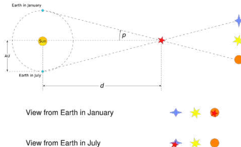
Figure 18.7: Stellar Parallax
