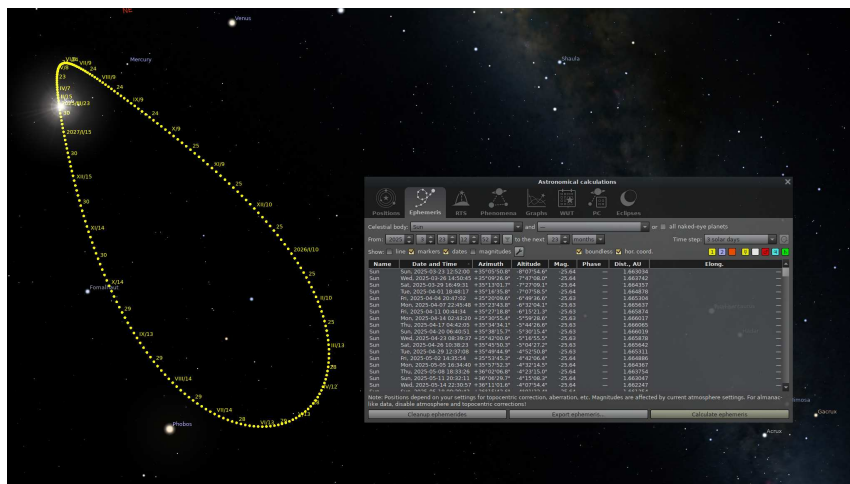
Figure 4.29: Astronomical Calculations (AstroCalc): Analemma on Mars
